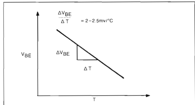
Figure 2. Change in VBE With Temperature
