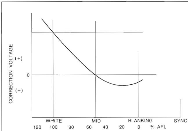
Figure 5. Medium Time Constant Correction Voltage Curve
