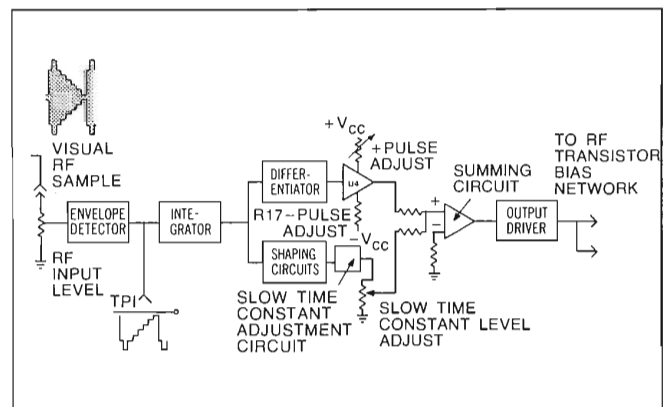
Figure 4. Differential Gain/APL Corrector Simplified Block Diagram
