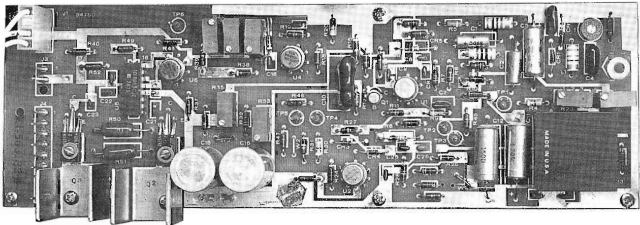
Figure 6. Printed circuit corrector board
